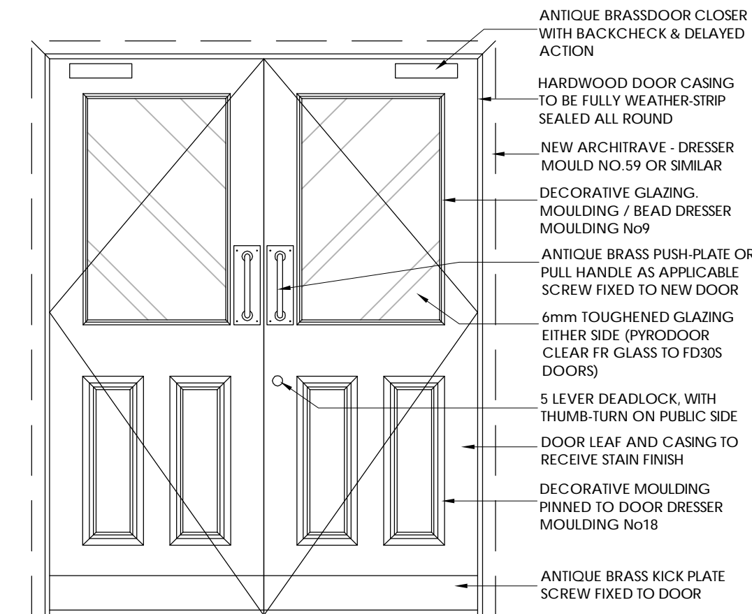
DOOR TYPE B - ENTRANCE LOBBY
