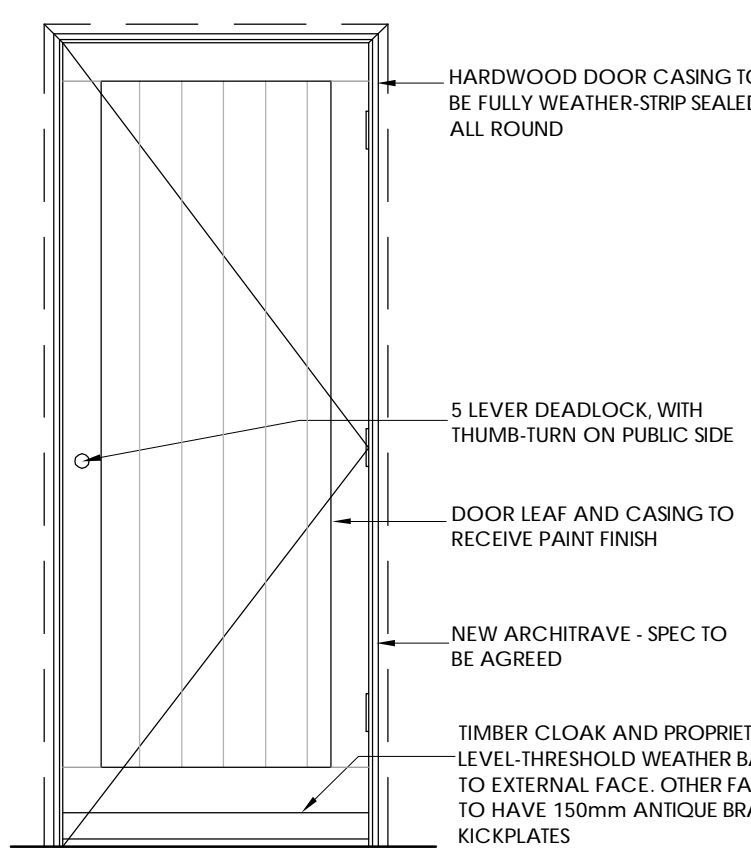
DOOR TYPE E - EXTERNAL KITCHEN DOOR
