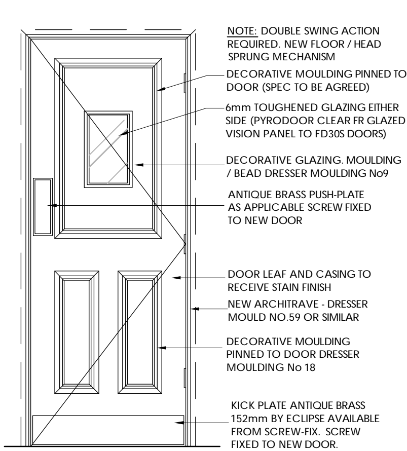
DOOR TYPE C - BETWEEN KITCHEN/TRADE
