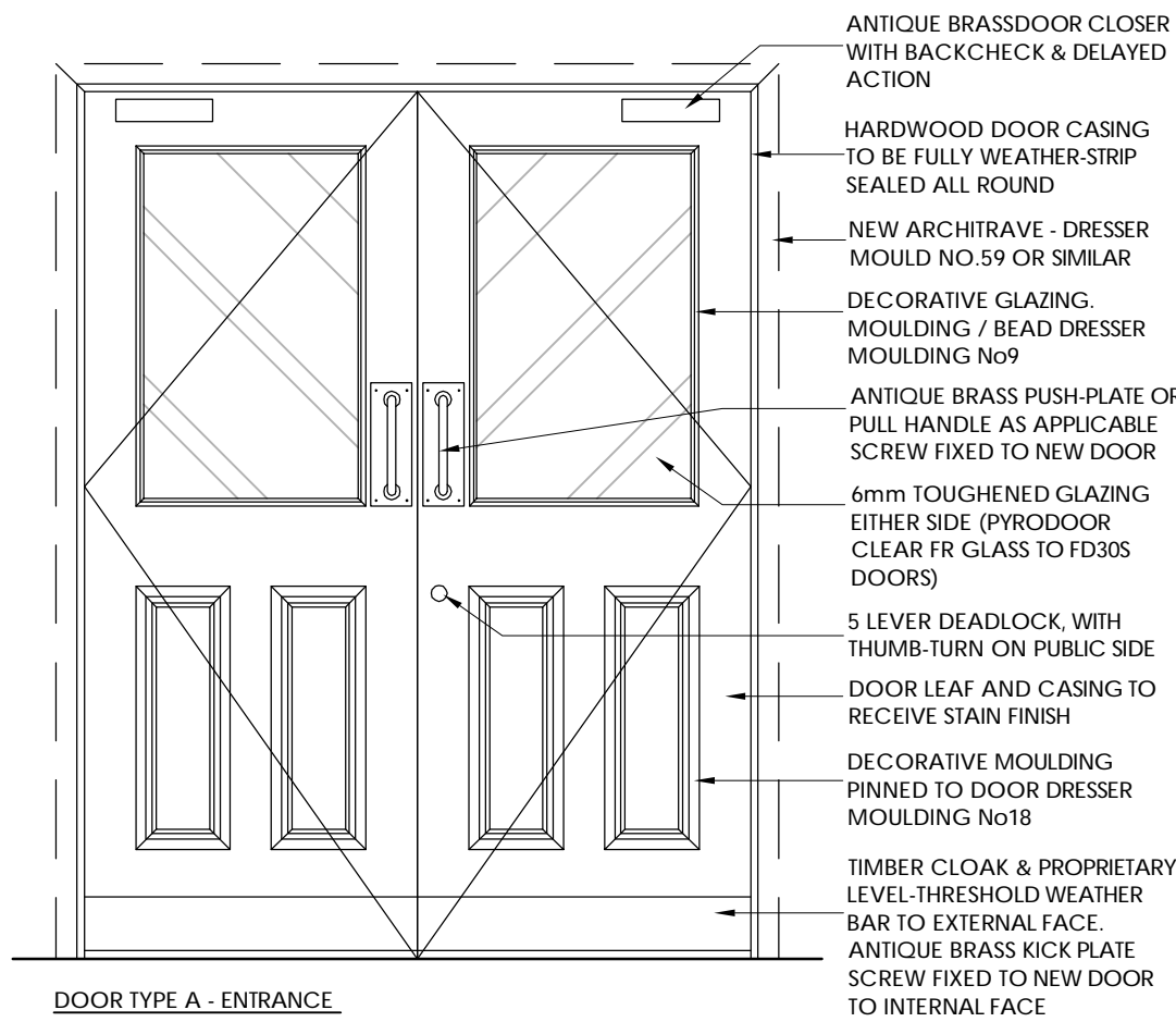
DOOR TYPE A - ENTRANCE
