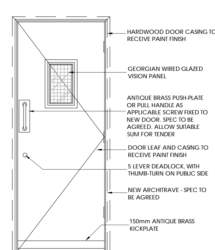
DOOR TYPE D - INTERNAL KITCHEN DOOR
