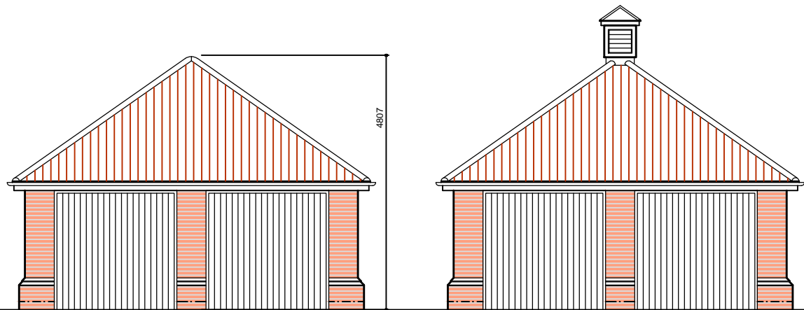
Standard type Proposed Front Elevation
