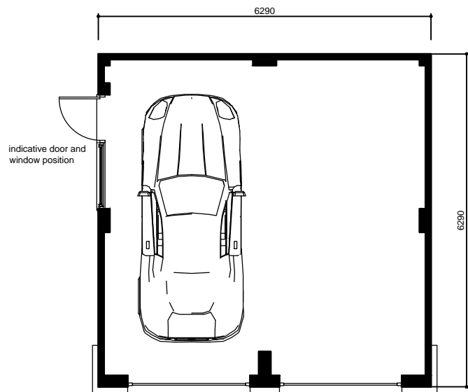
Proposed Double Garage floor layout
