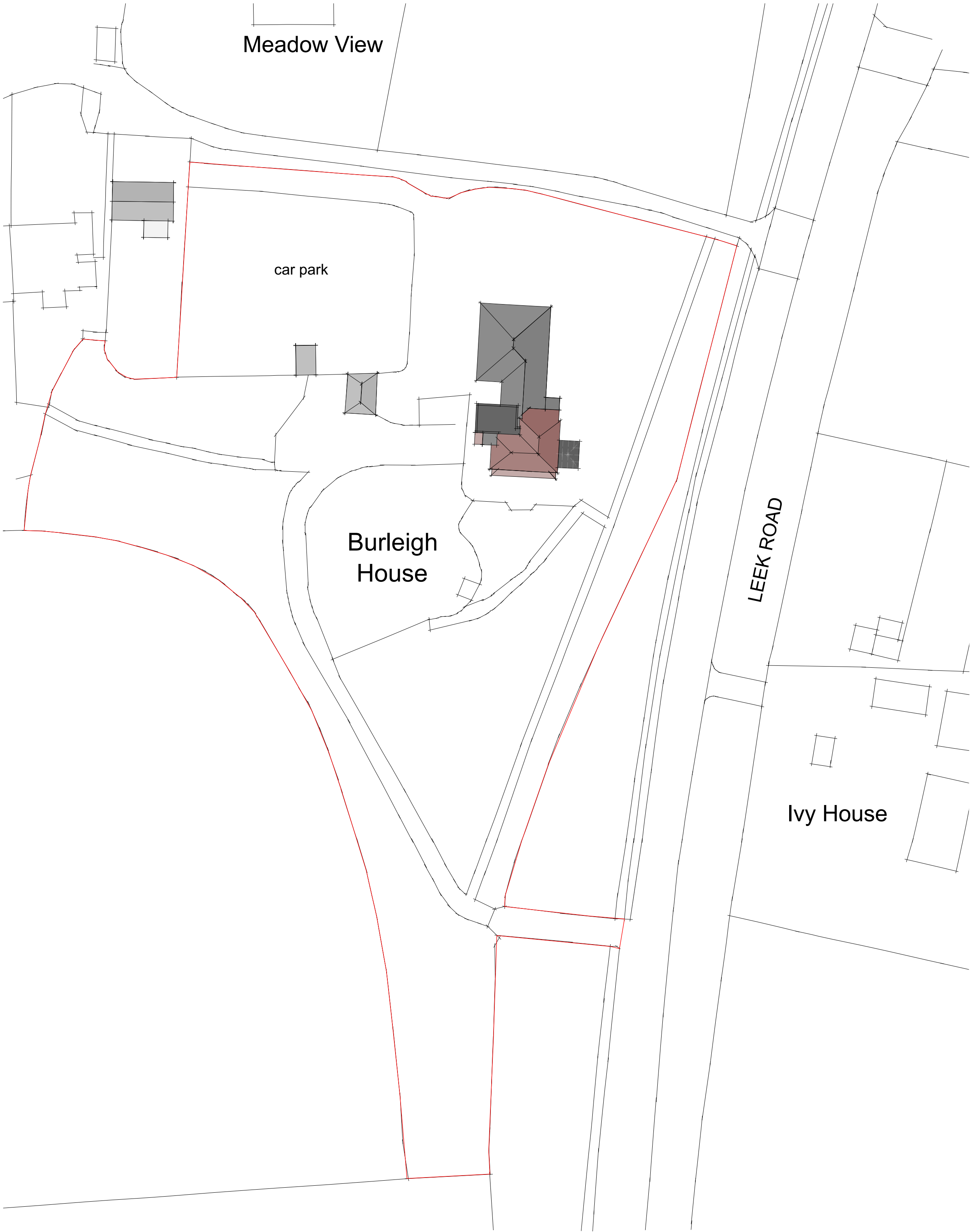
BLOCK PLAN AS PROPOSED Scale 1:500 @ A1
