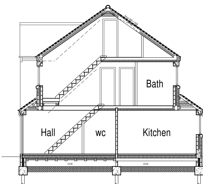
Typical Section
