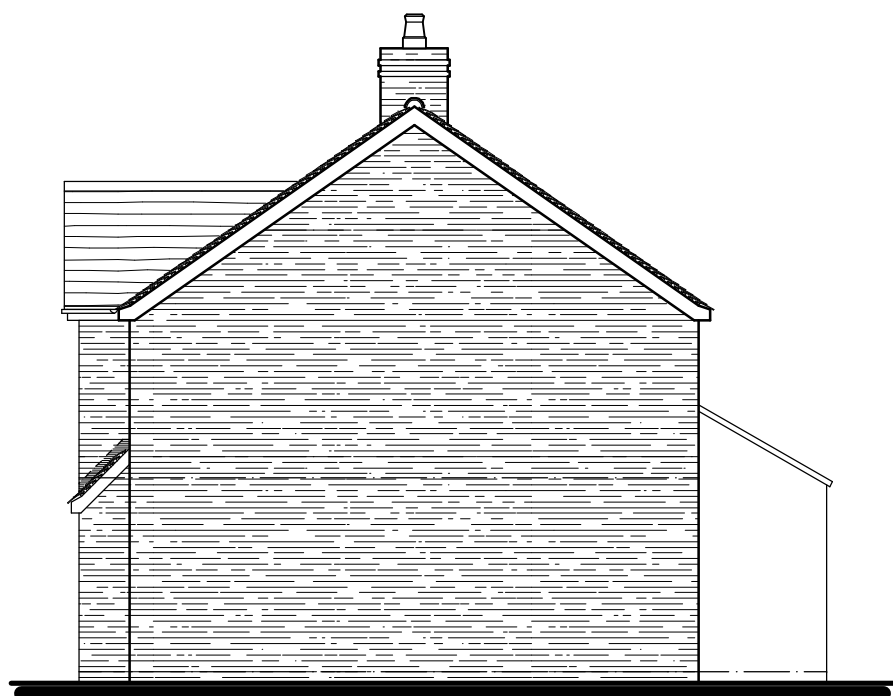
East Elevation
