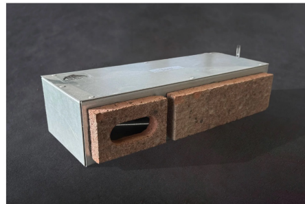
Brick Slip Facing 50mm Cavity
