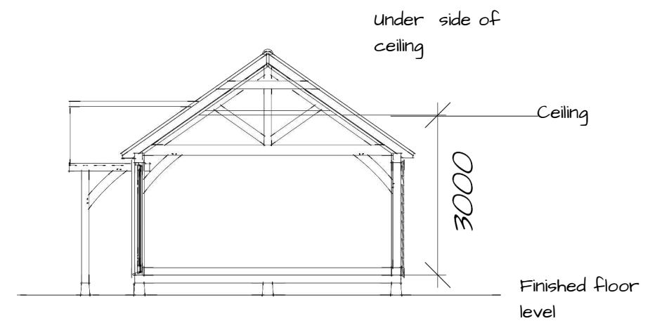
Proposed Cross Section
