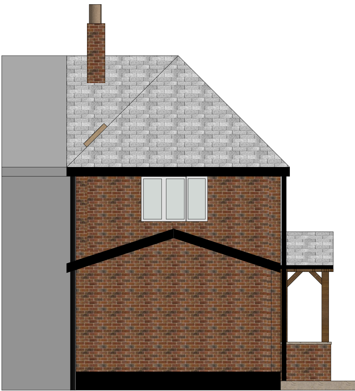
SMD/2026/0018 SIDE ELEVATION 1:50
