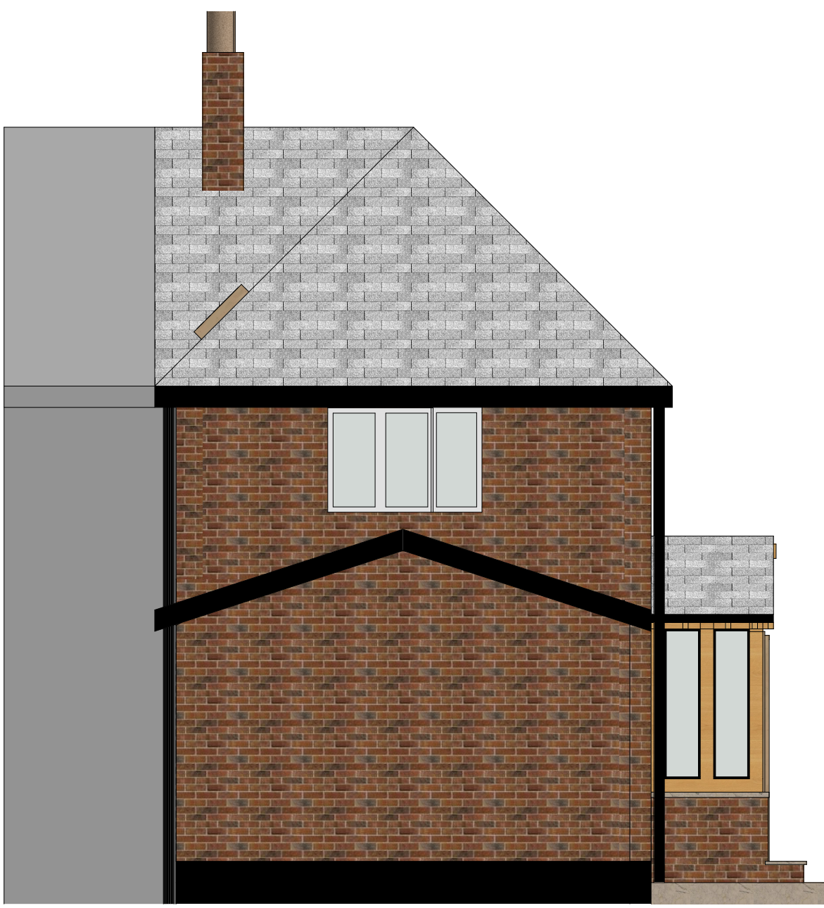
AMENDED PROPOSED SIDE ELEVATION 1:50
