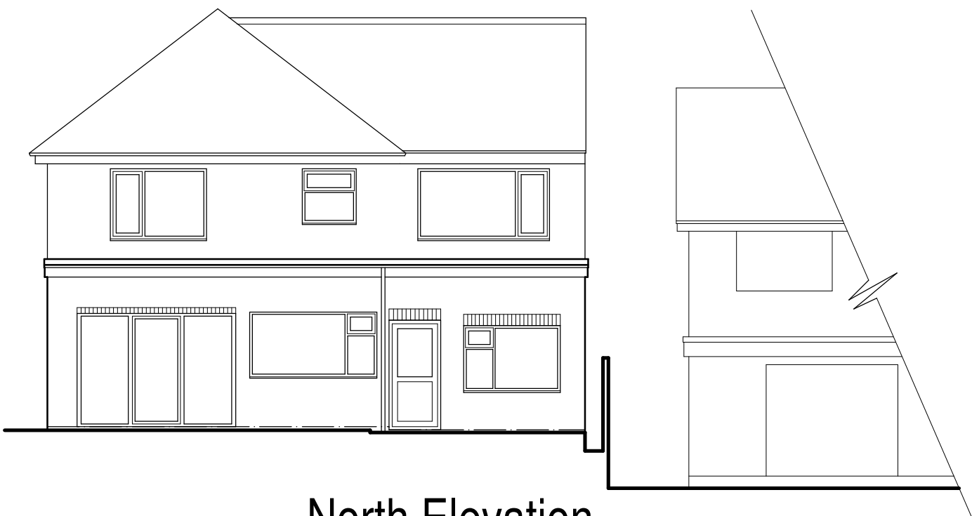
North Elevation
