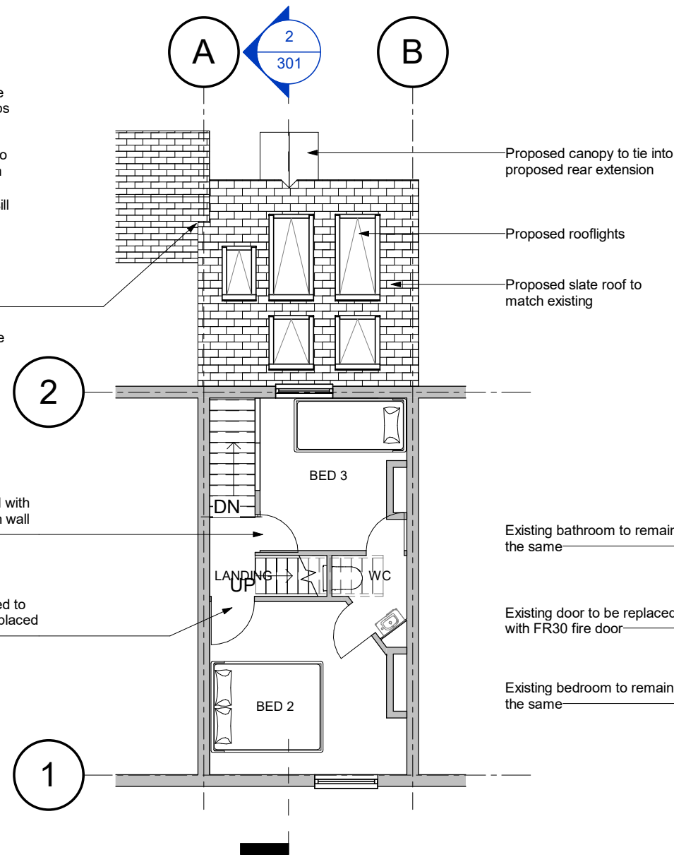
Level 1 - Proposed 1 : 100
