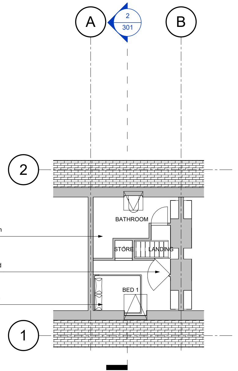
Level 2 - Proposed 1 : 100
