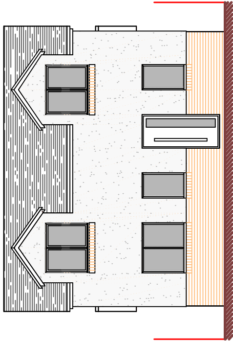
Front (North) Elevation
