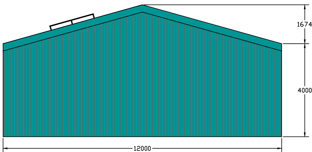
Southeast Gable Elevation
