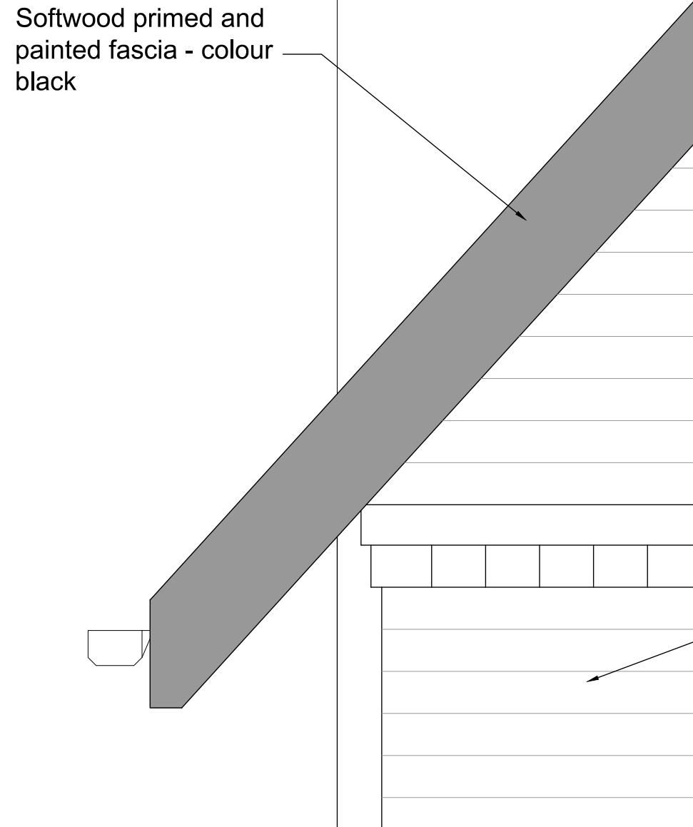
EAVES AREA DETAIL SCALE 1:10
