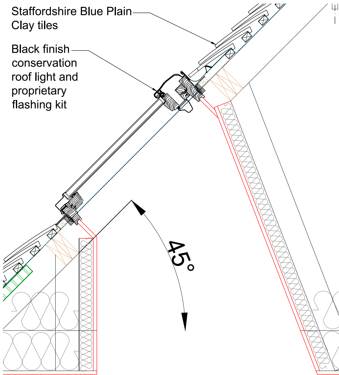
Conservation Rooflight Section A-A SCALE 1:5
