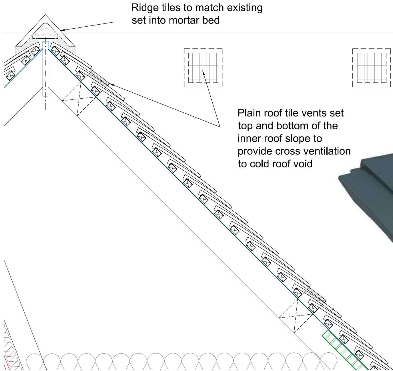
Plain Clay Tile Roof Vents Set on the inner slope side SCALE 1:10
