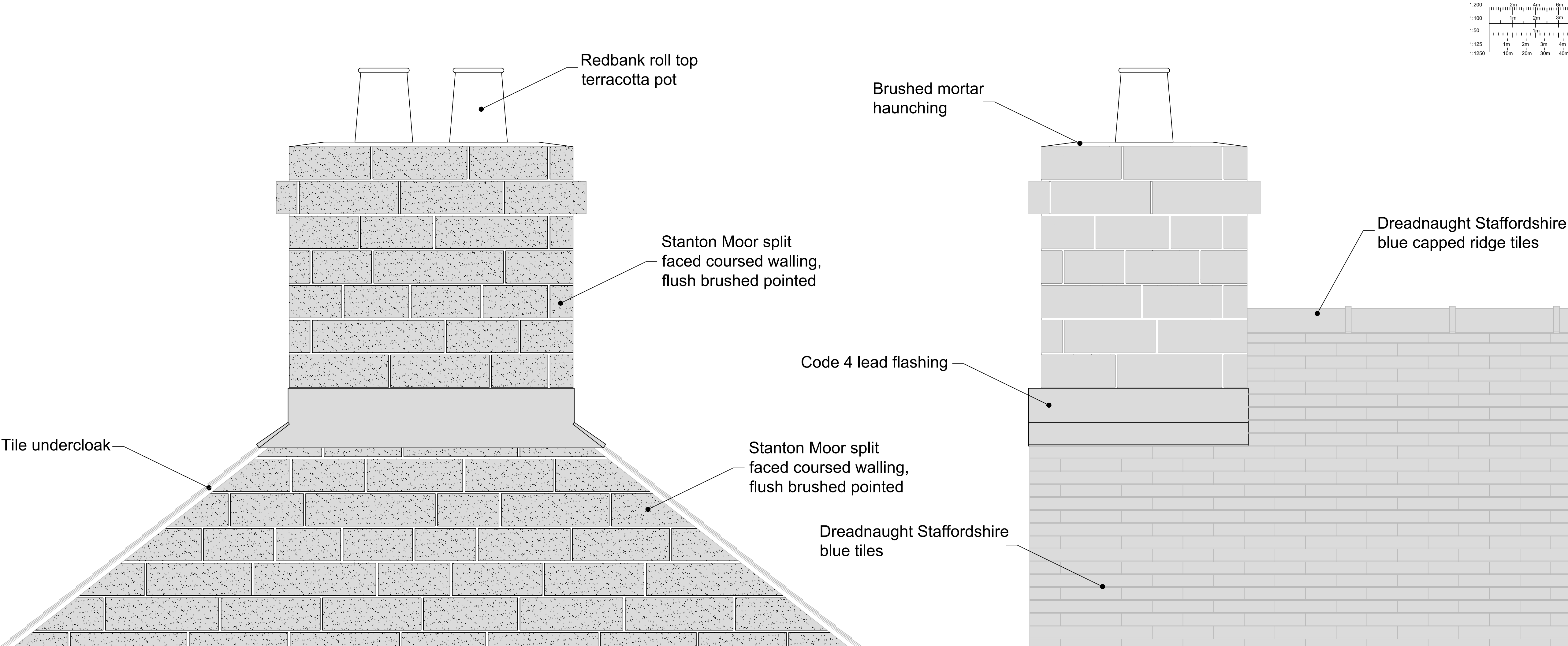
Roof Detail Around Chimney
