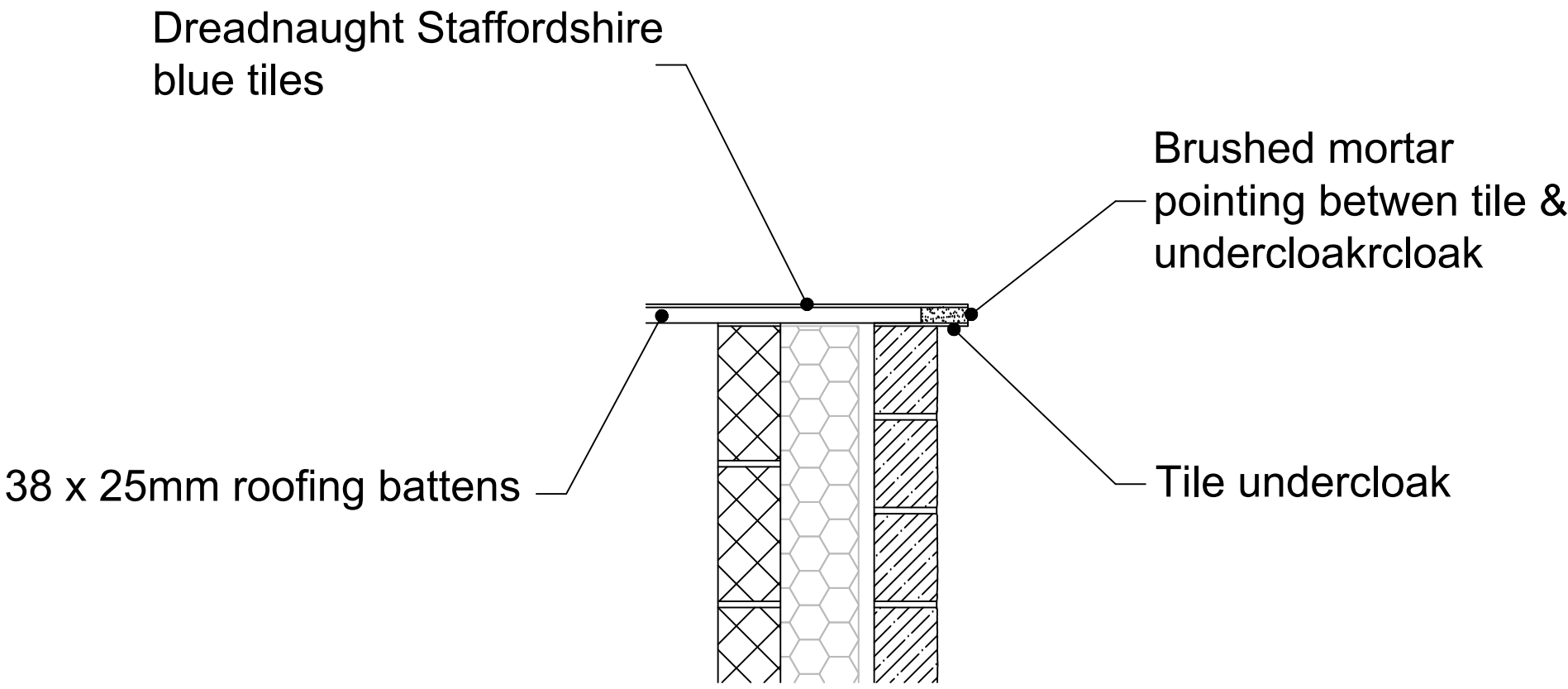
Typical Verge Section
