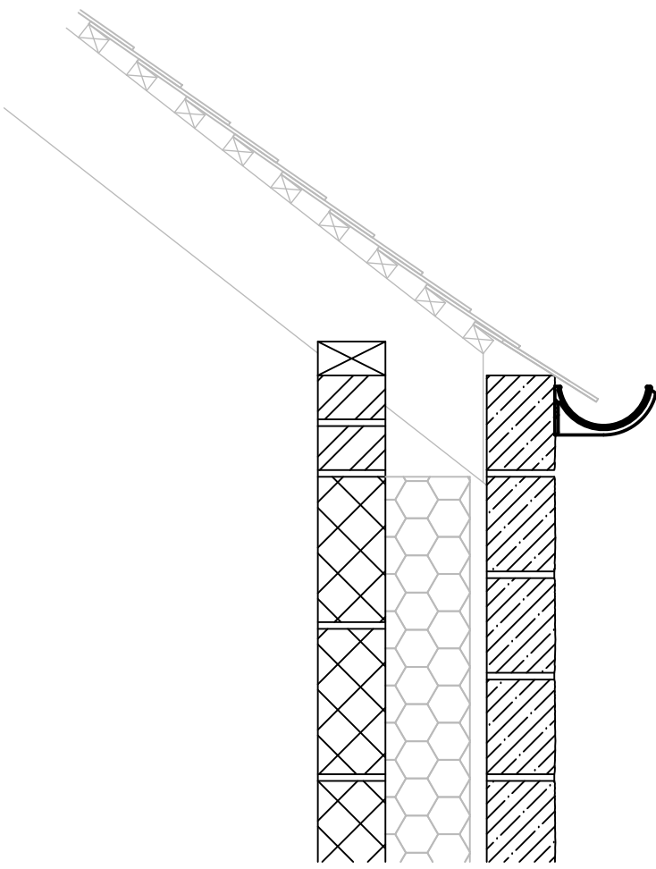
Typical Eaves Section
