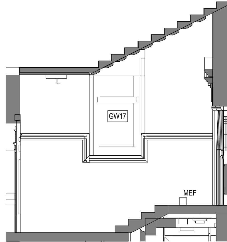
G0010 - Elevation D 1 : 50
