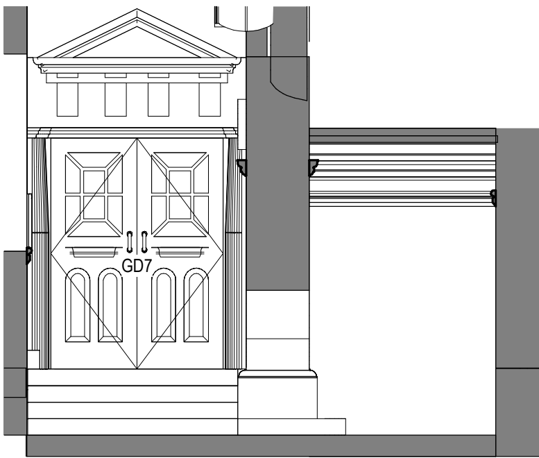
G0010 - Elevation A 1 : 50
