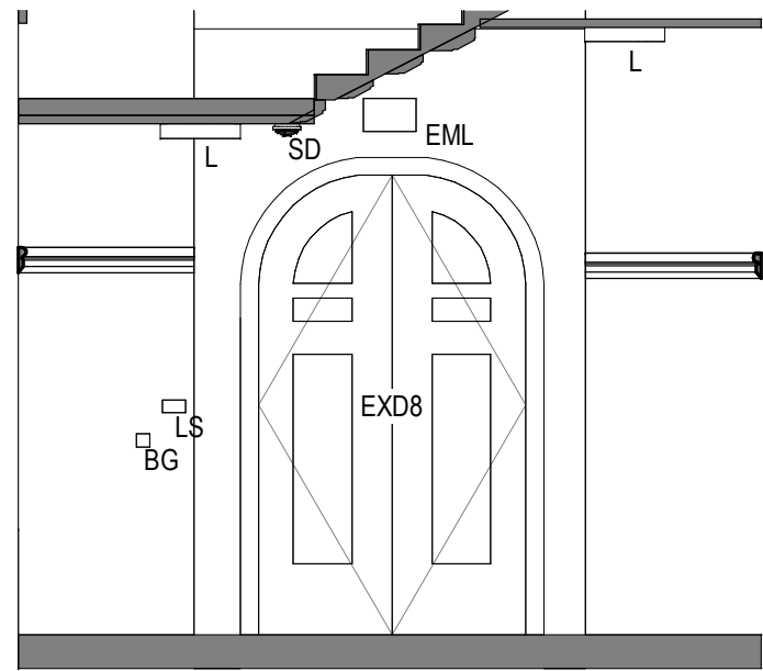
G0010 - Elevation C 1 : 50
