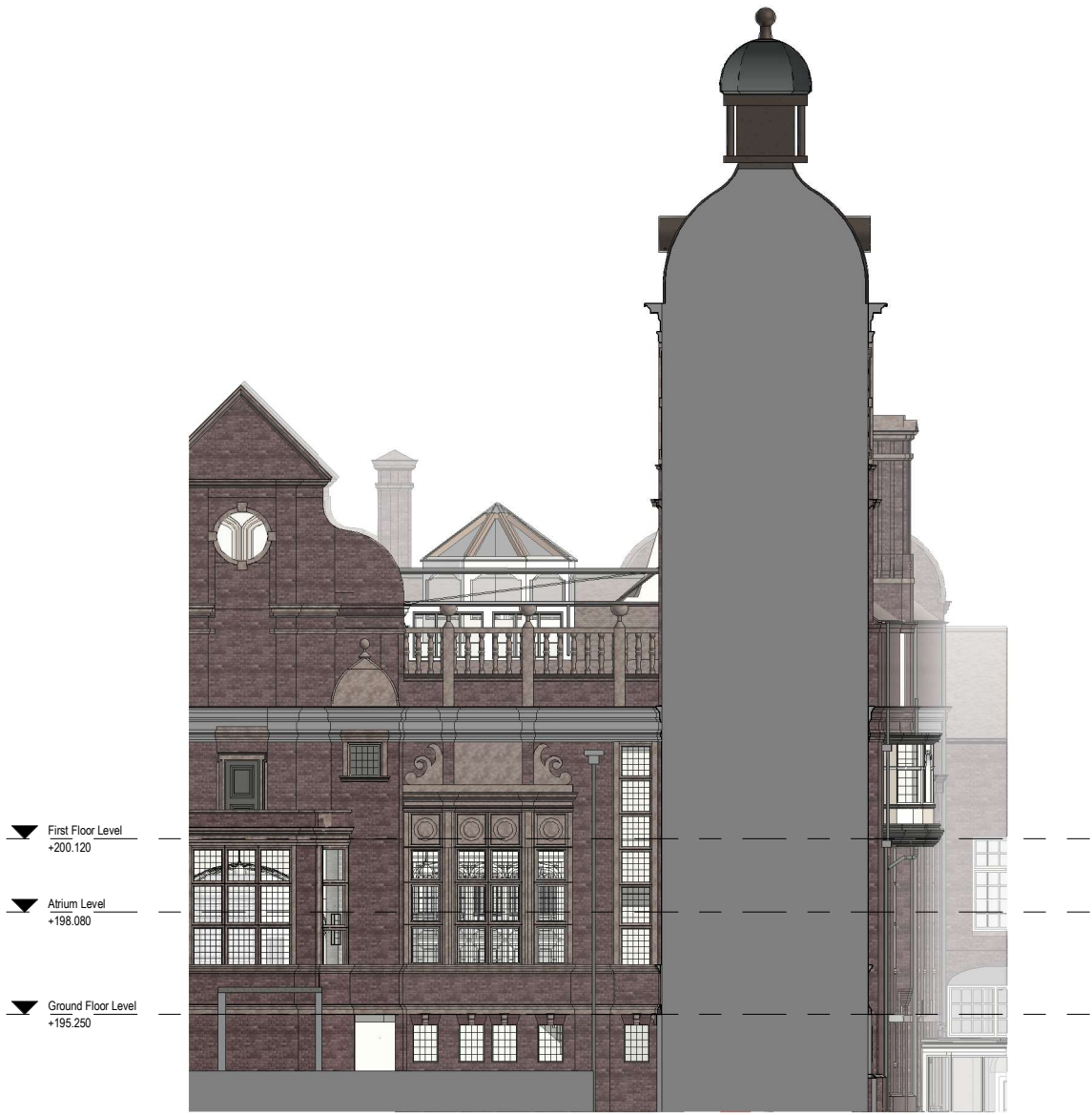
1 Existing South Elevation - 1 1 : 100
