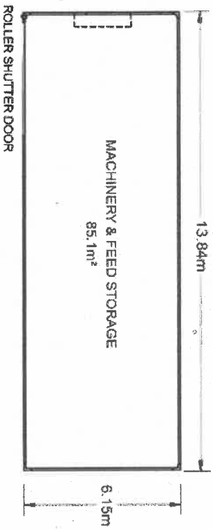
FLOOR PLAN 1:100
