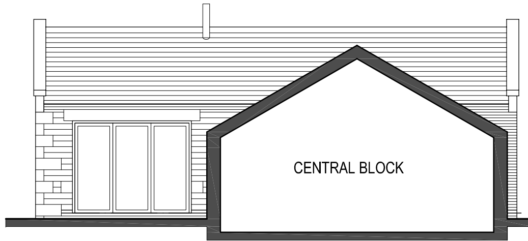
SECTION E-E
