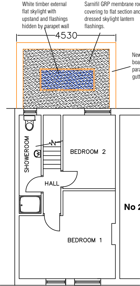
PROPOSED FIRST FLOOR PLAN, 1:100
