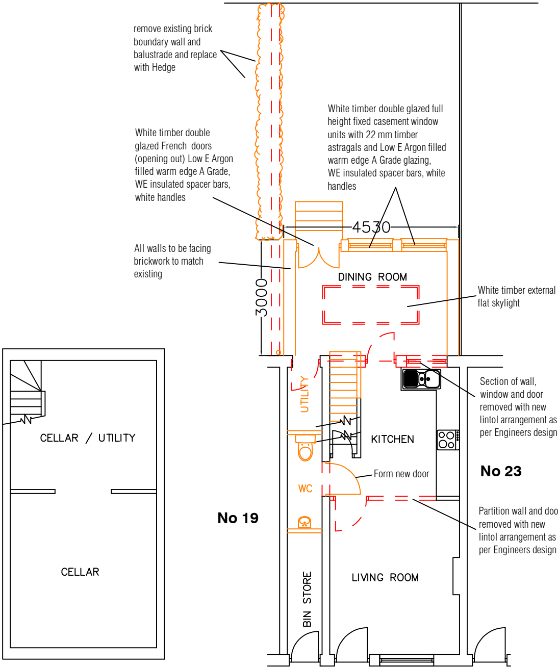
PROPOSED BASEMENT FLOOR PLAN, 1:100
