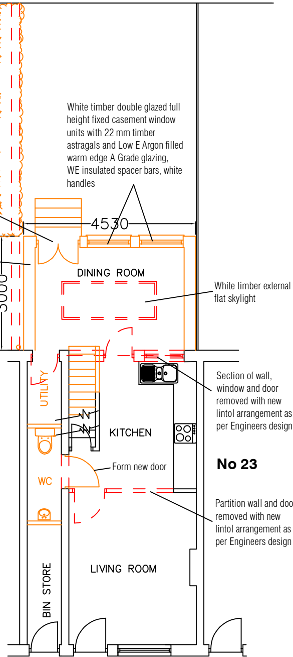
PROPOSED GROUND FLOOR PLAN, 1:100
