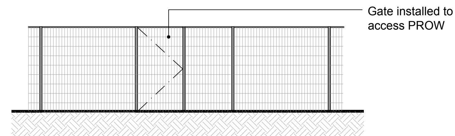
PROPOSED FENCE & GATE ELEVATION
