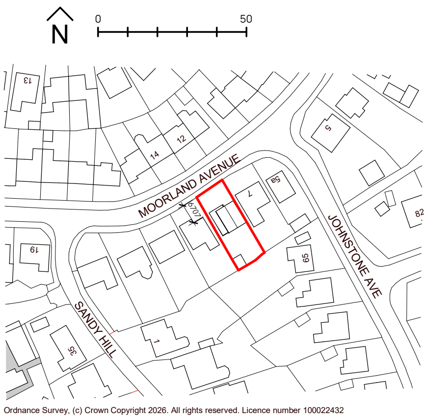
Location Plan 1 : 1250
