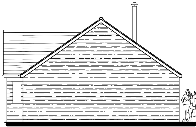
West Elevation
