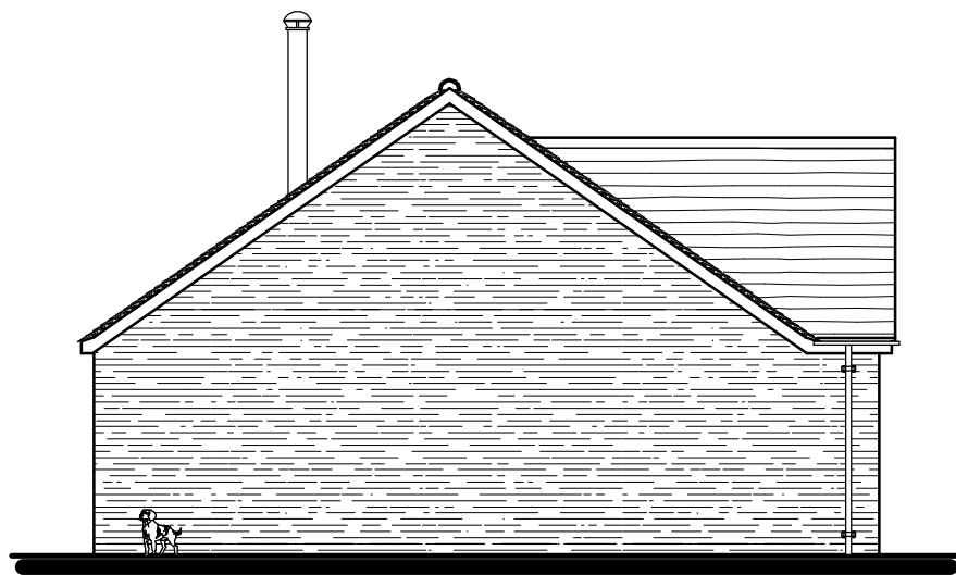
East Elevation
