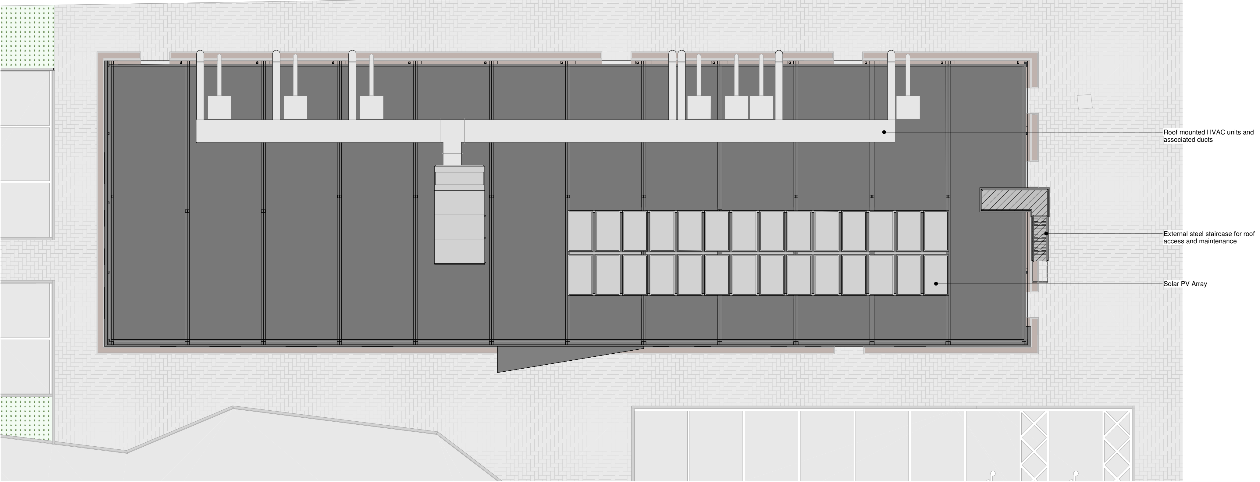
Roof Plan as Proposed 1 : 100
