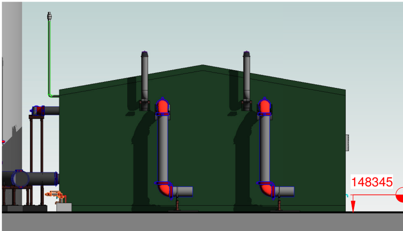
Elevation C (North Elevation) 1 : 100
