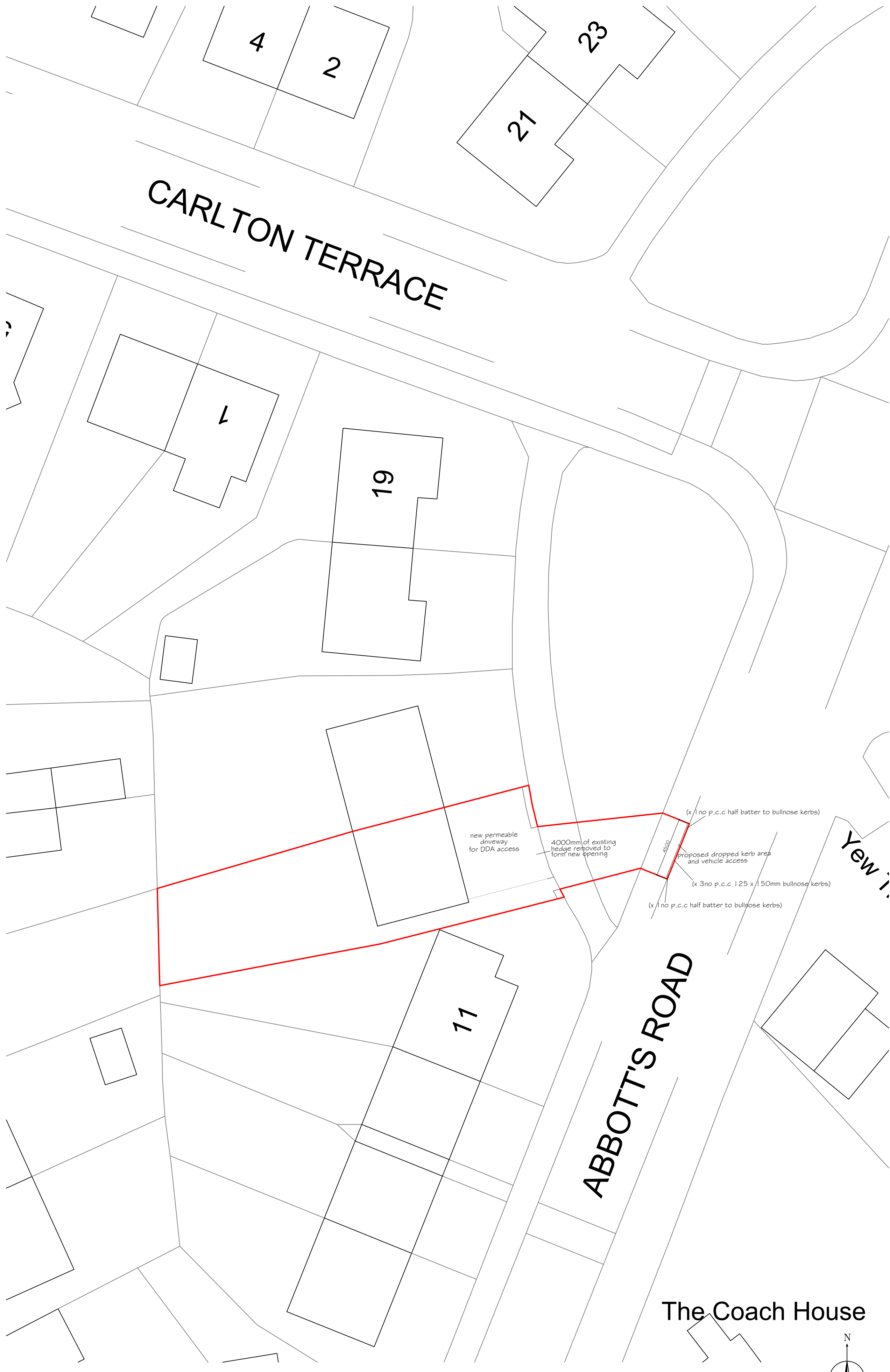
Proposed Site Layout Plan- 1 : 200
