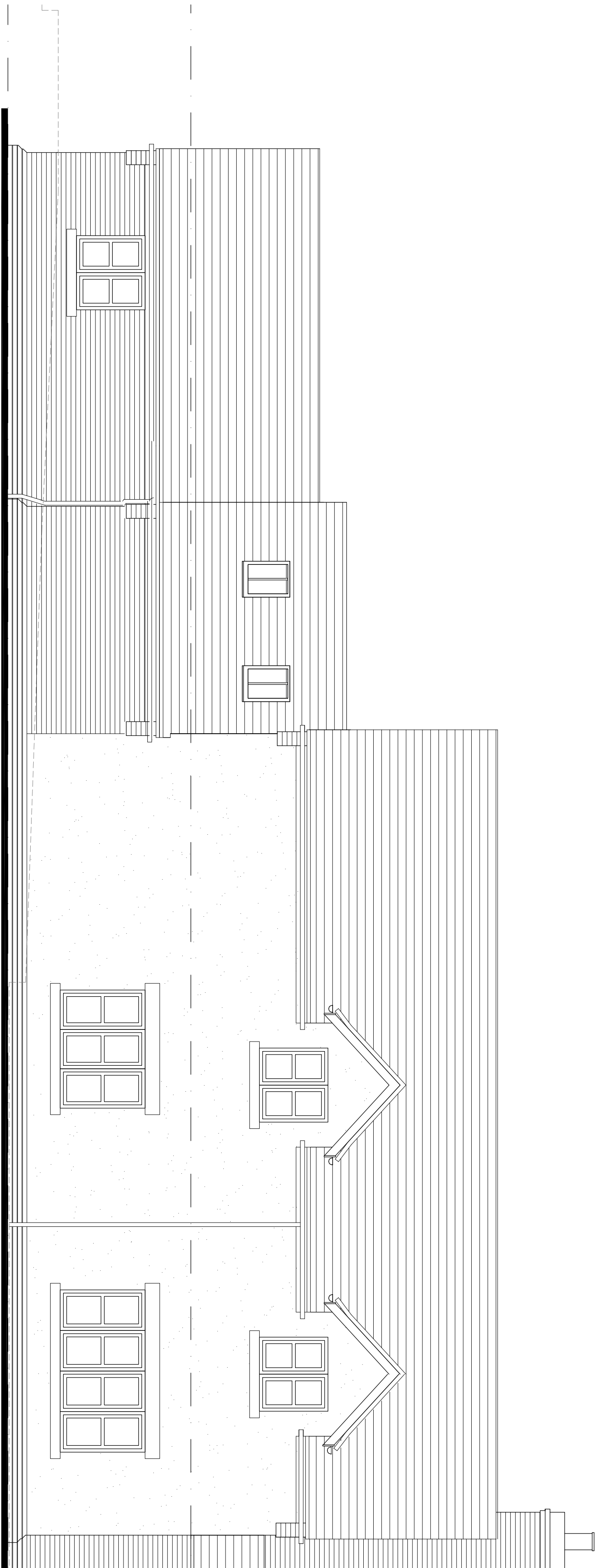
SIDE ELEVATION 1:50
