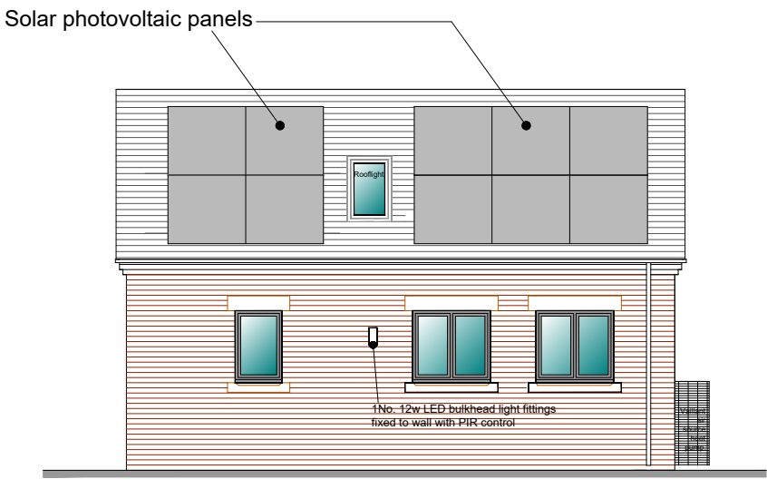
West Elevation
