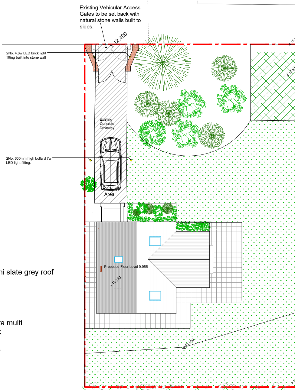
Details of Driveway Lighting scale 1:200 @ A2 First Floor Plan
