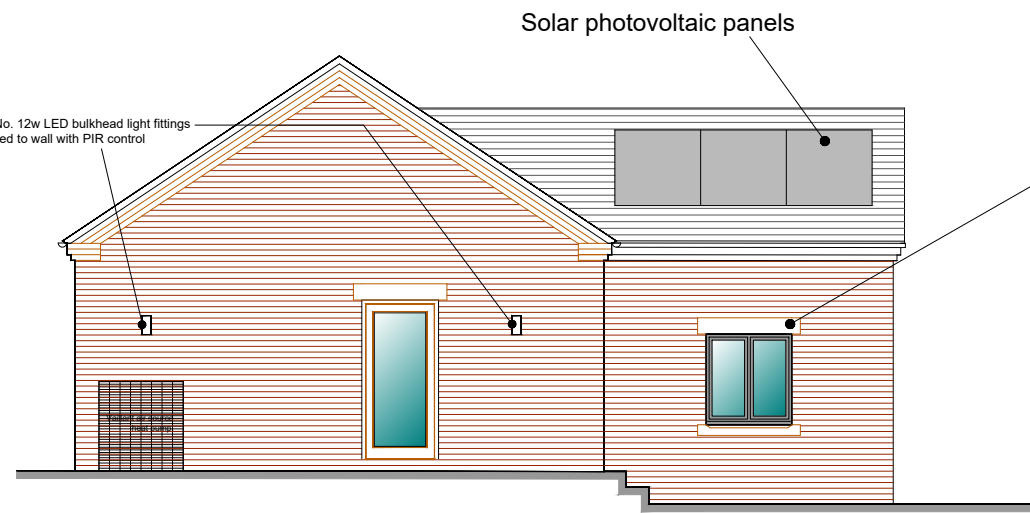
South Elevation
