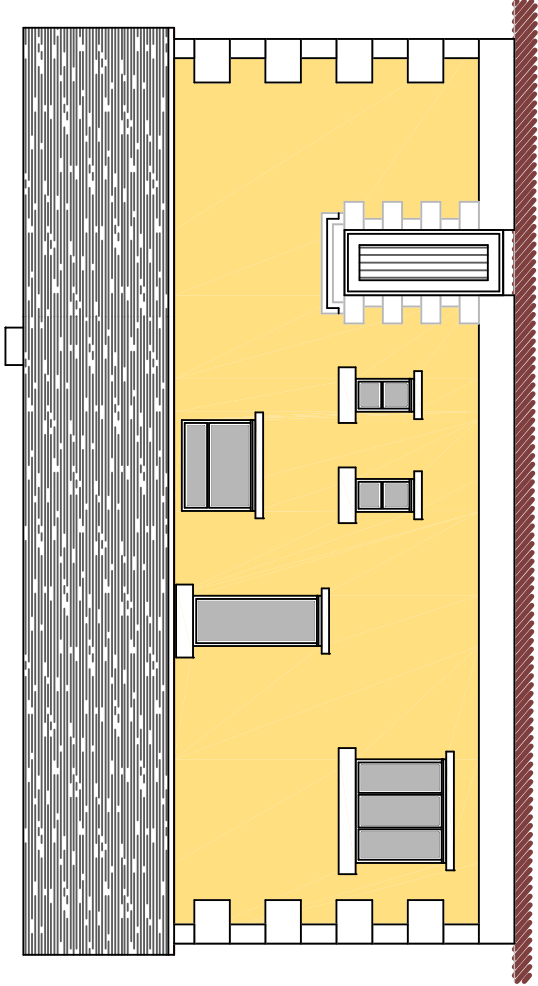
Rear Elevation
