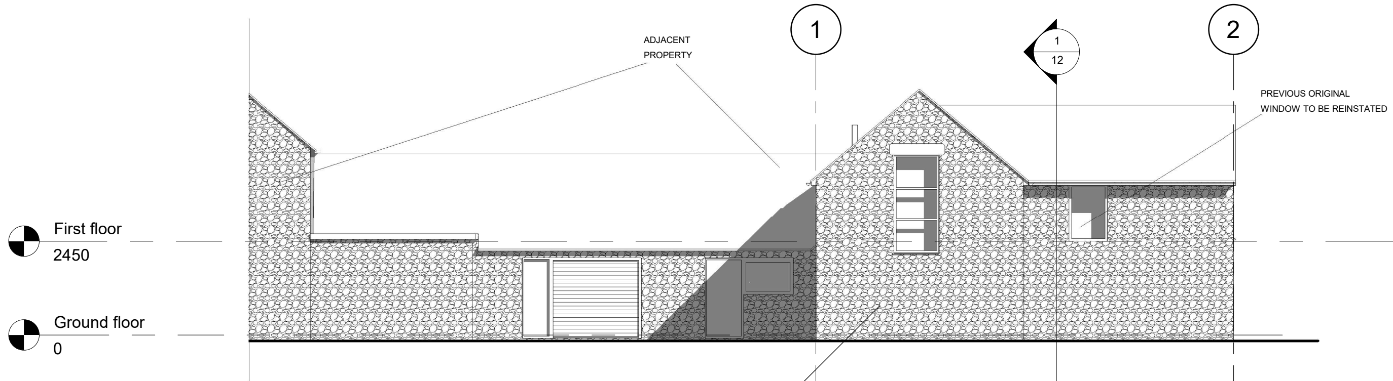
SOUTHEAST ELEVATION
