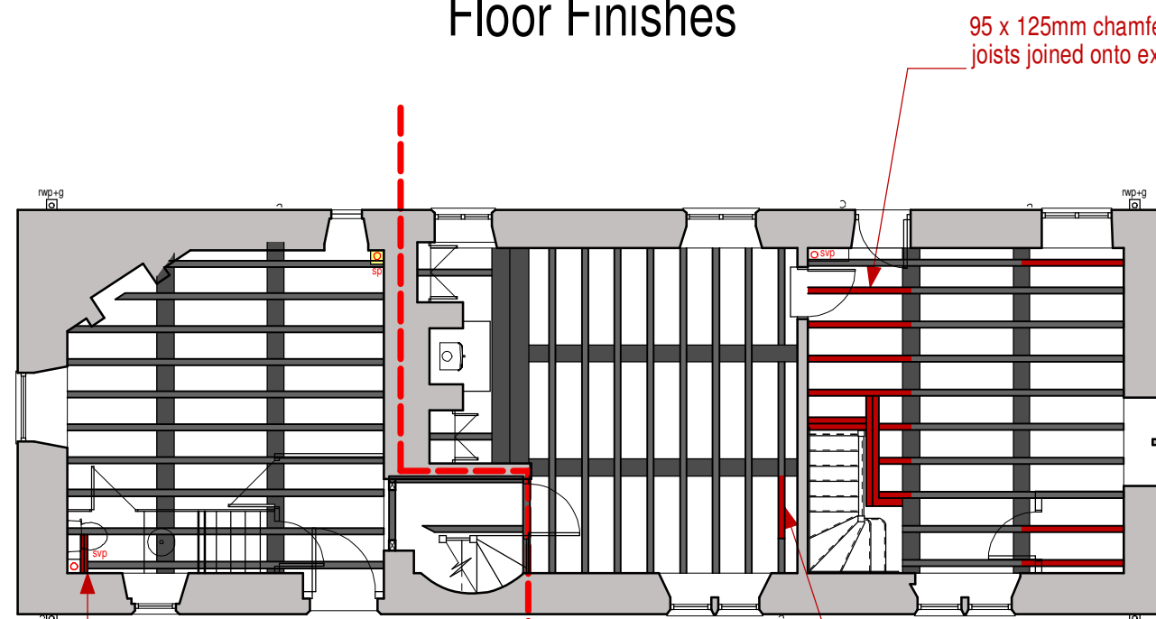
First Floor Joist Plan
