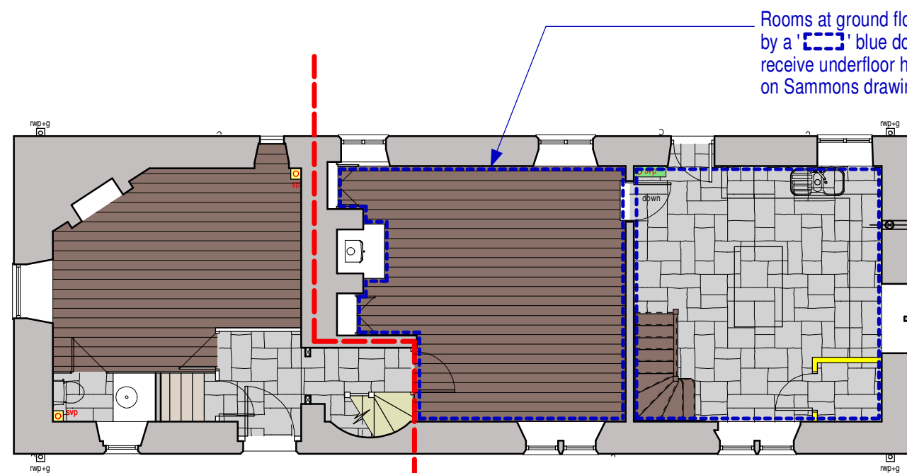
Ground Floor Plan Floor Finishes
