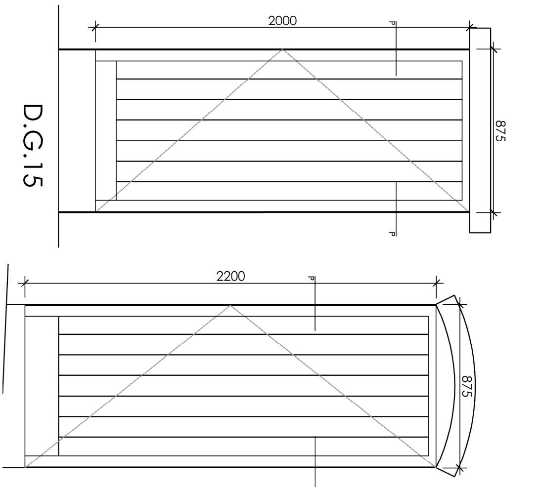
Elevations 3 scale 1:100
