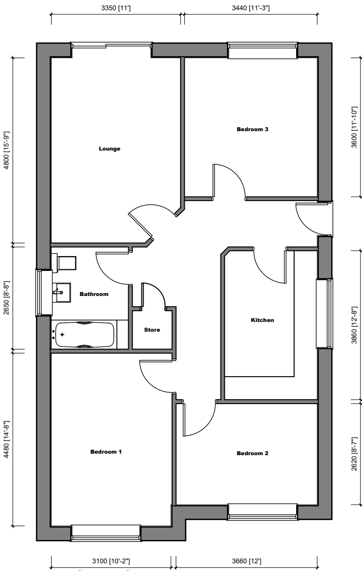
Floor Plan
