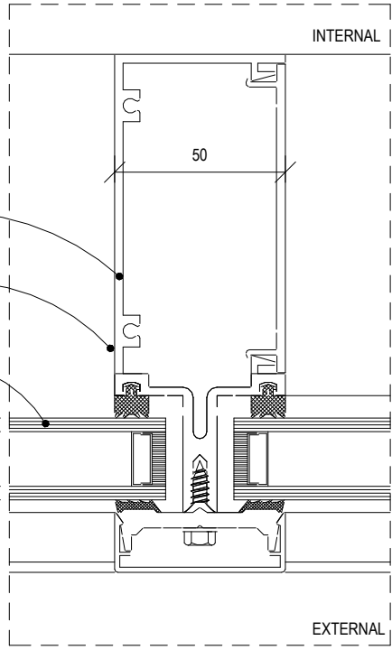
Detail 4: Mullion 1:2
