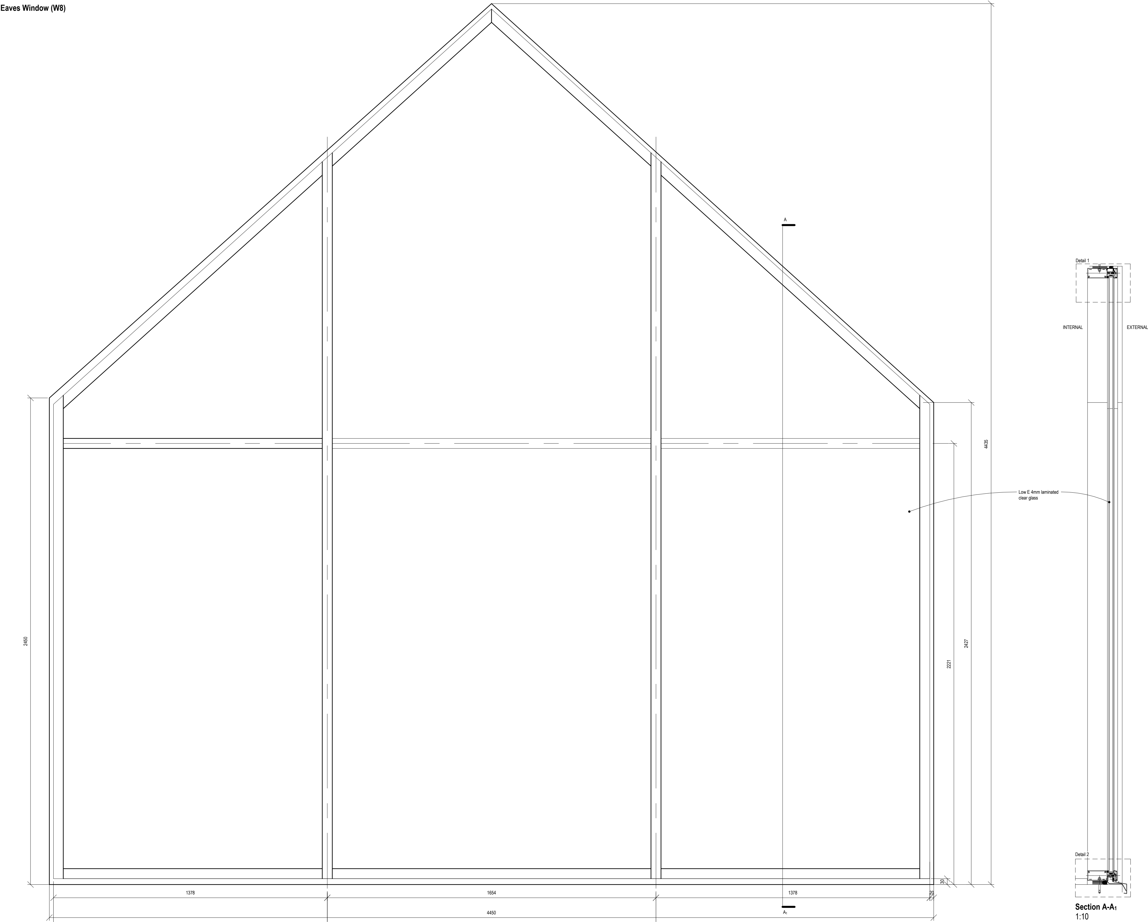
External Elevation 1:10
