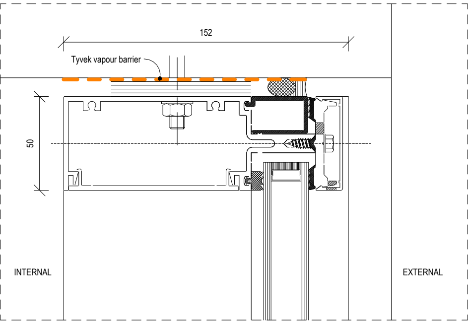
Detail 1: Head 1:2
