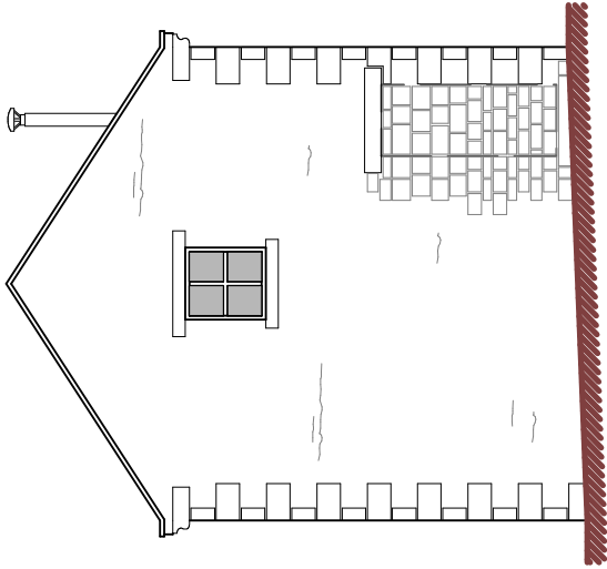
Side elevation (West)
