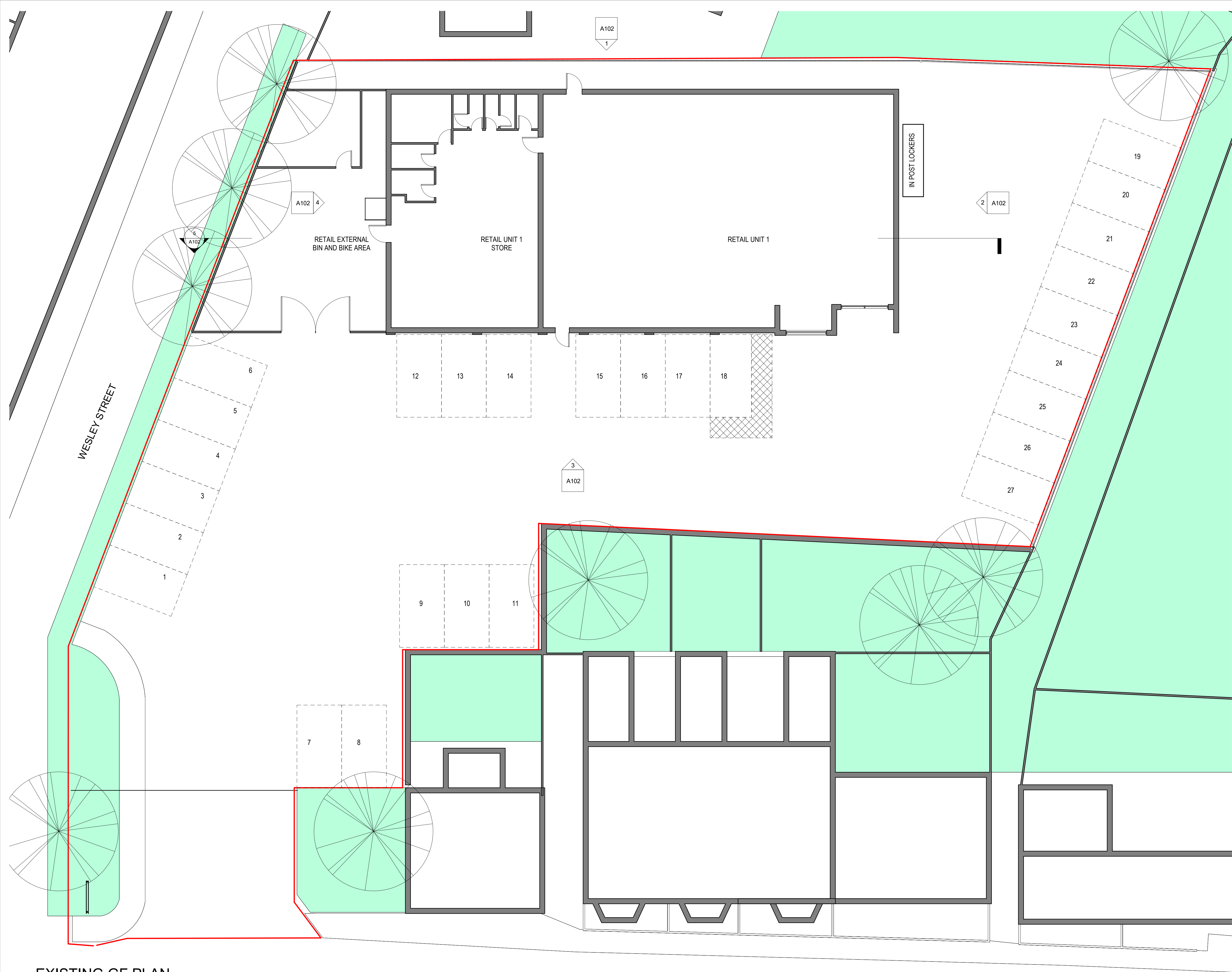
1 EXISTING GF PLAN 1 : 100
