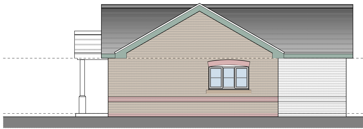
side elevation
