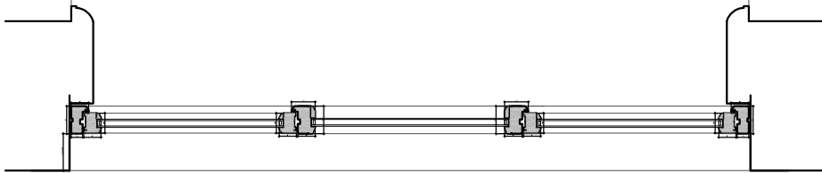
WINDOW PLAN 1:20
