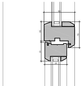
DETAIL B 1:5
