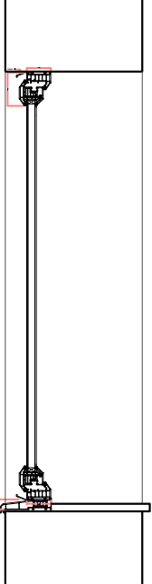
WINDOW SECTION 1:20
