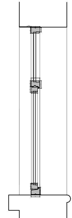
WINDOW SECTION 1:20
