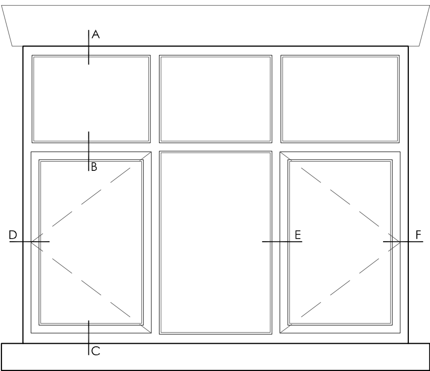
WINDOW ELEVATION 1:20
