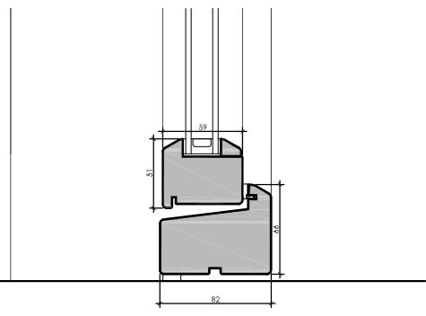
DETAIL C 1:5
