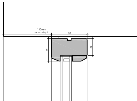
DETAIL A 1:5
