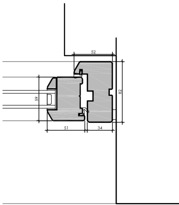
DETAIL F 1:5
