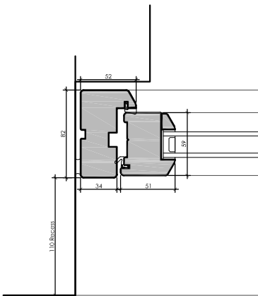
DETAIL D 1:5
