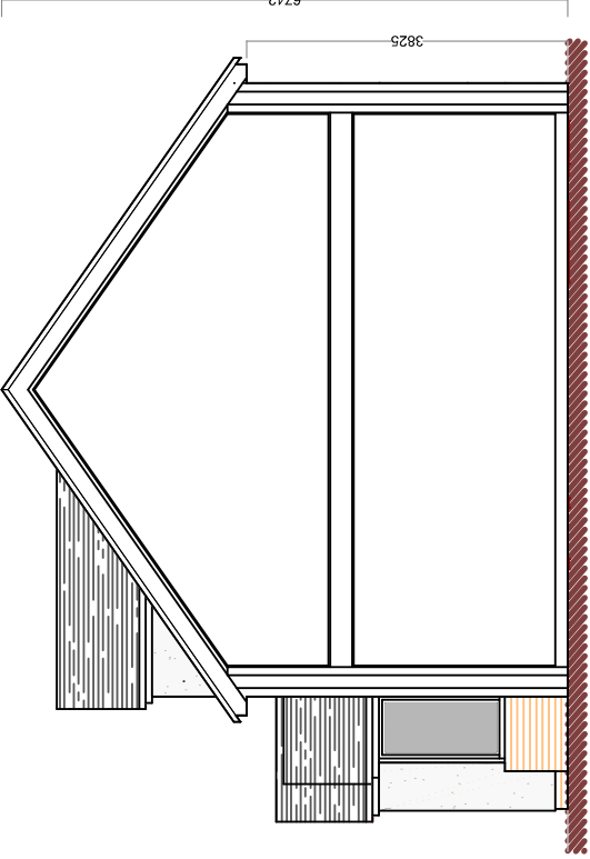
Indicative Section
