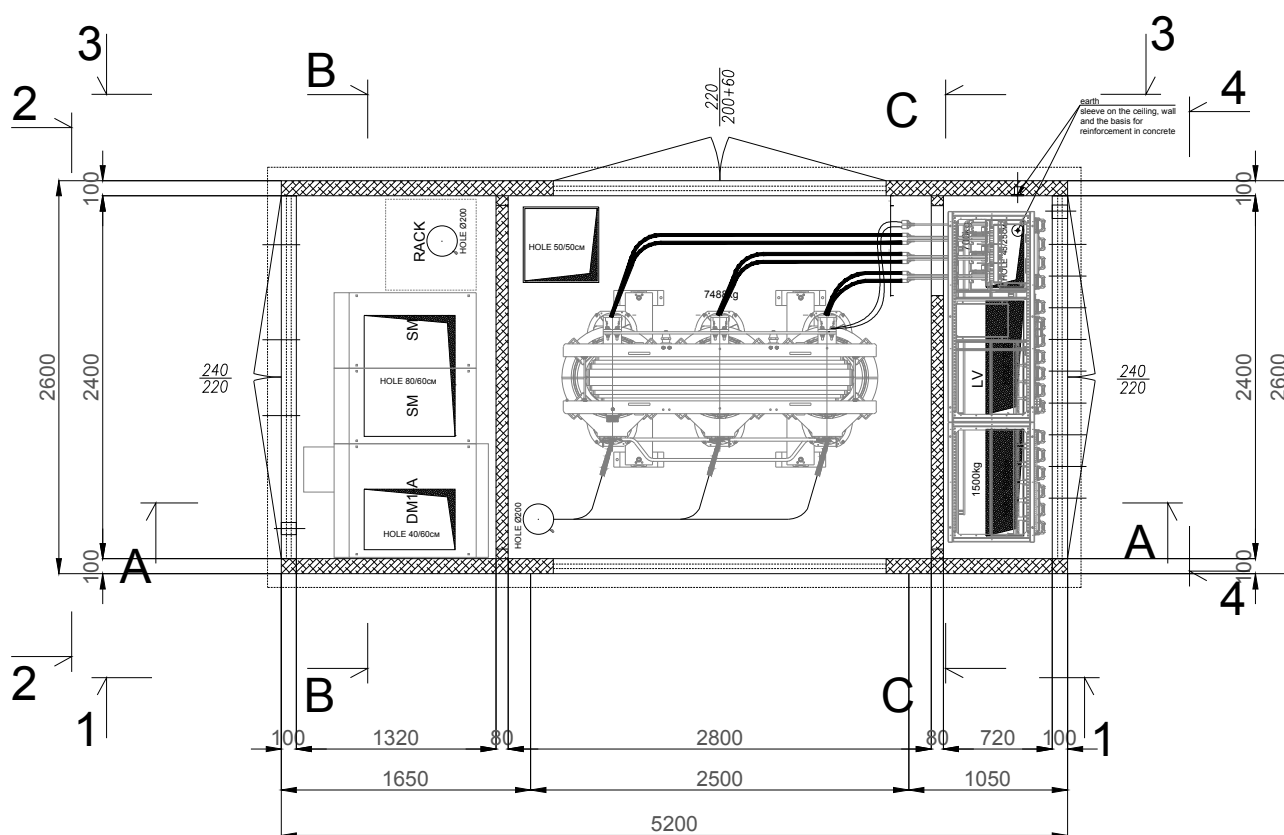
Transformer Station Elevations
