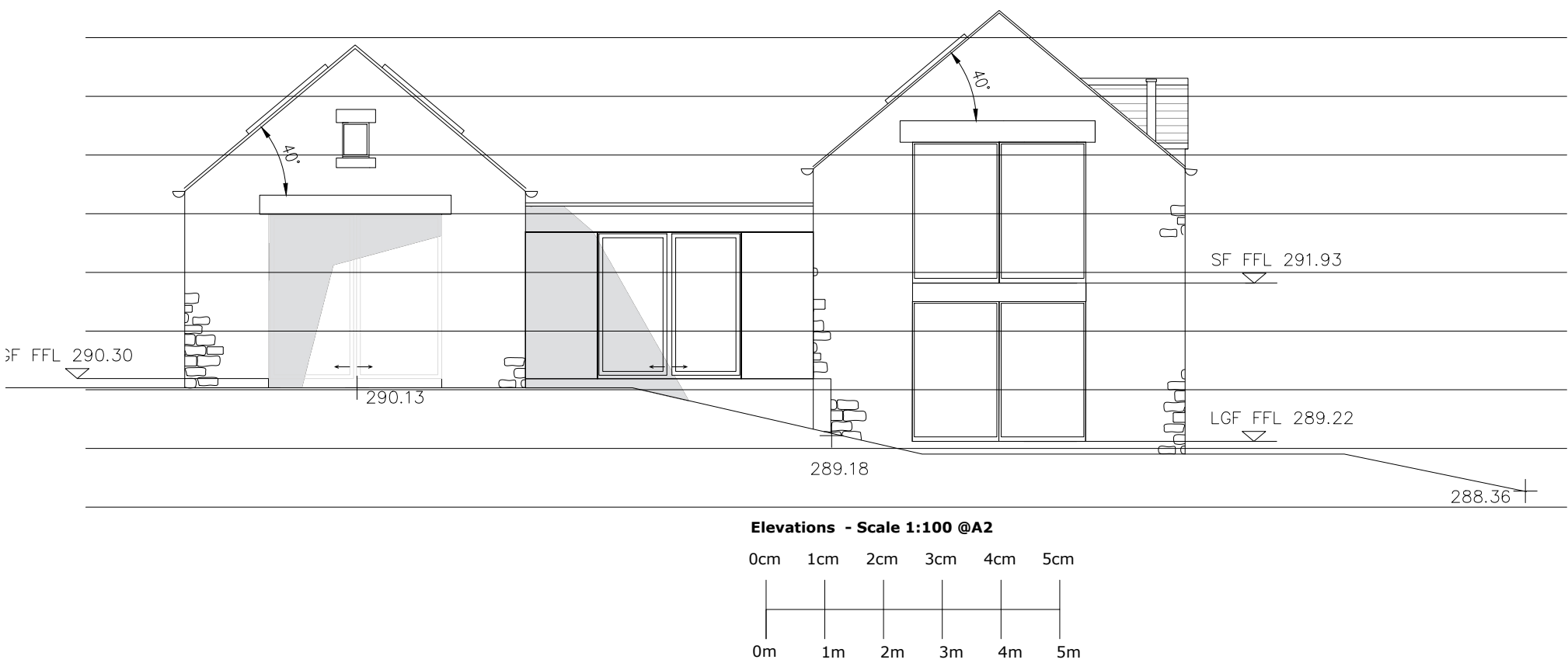
South Elevation
