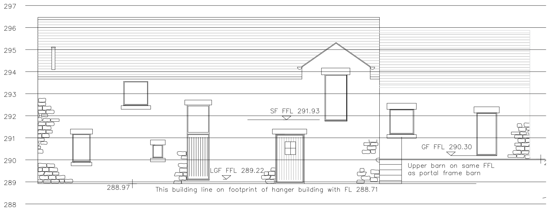
East Elevation
