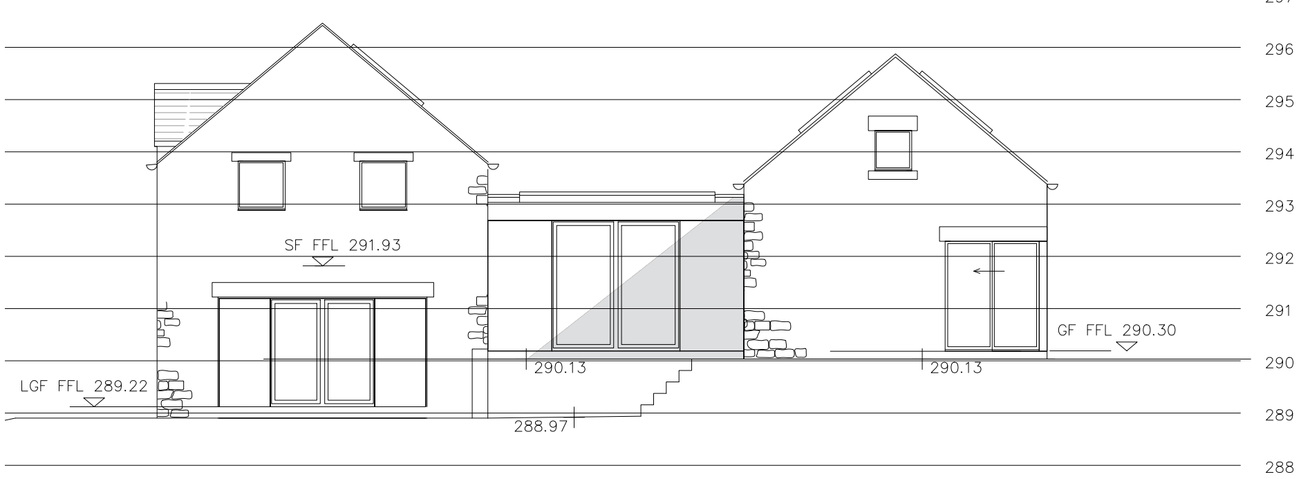
North Elevation
