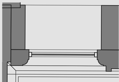
Plan GW21
