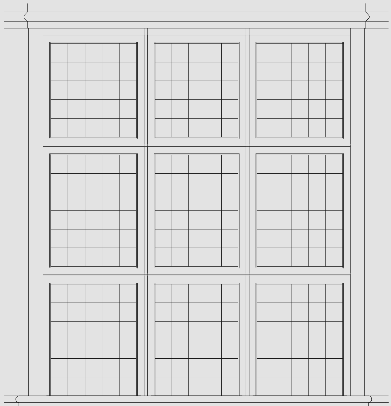
Elevation GW23
