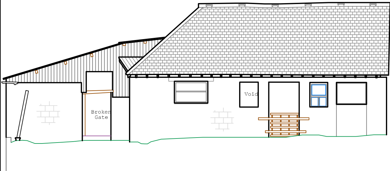
EXISTING ELEVATION 1
