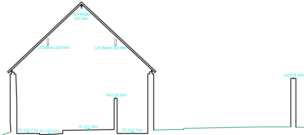
EXISTING ELEVATION 4
