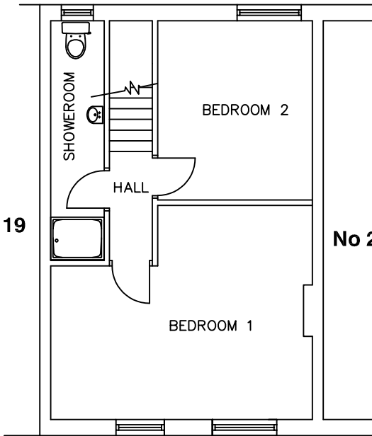
EXISTING FIRST FLOOR PLAN, 1:100
