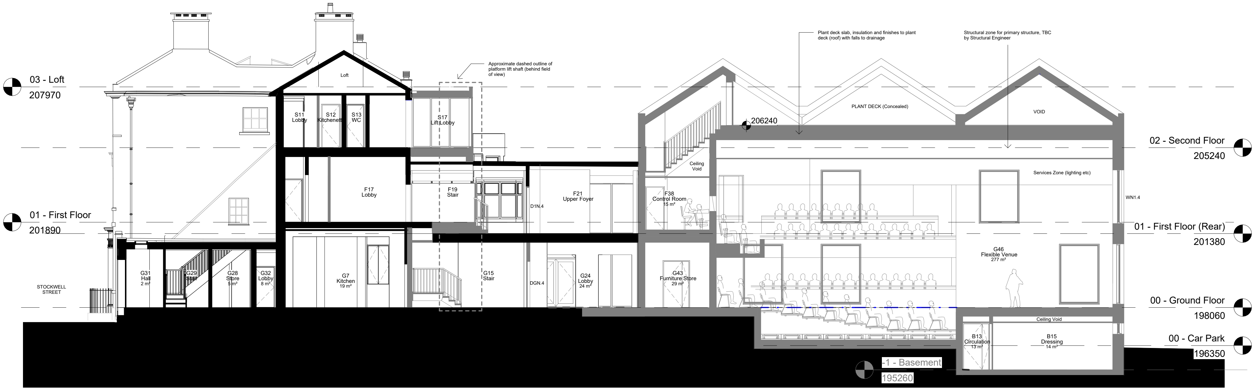
Section A-A as Proposed 1 : 100
