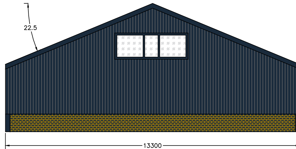
Northeast Gable Elevation
