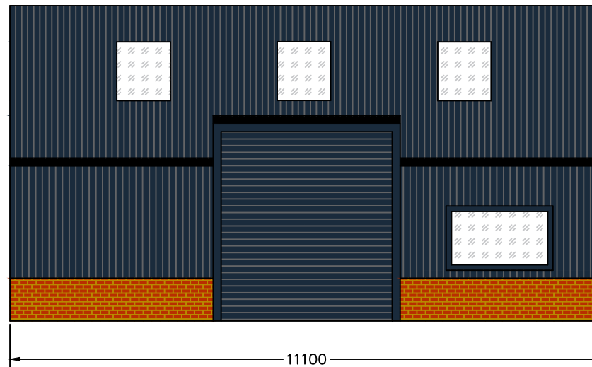
Northwest Side Elevation
