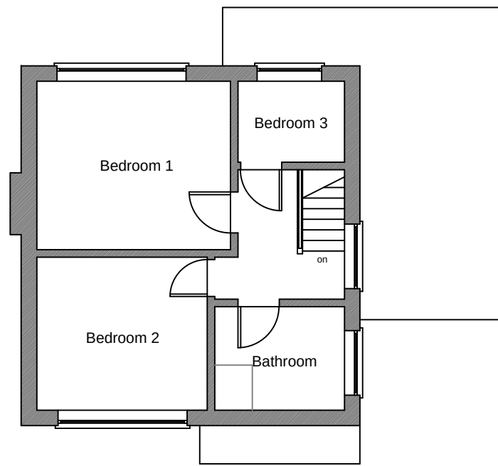
First Floor Layout
