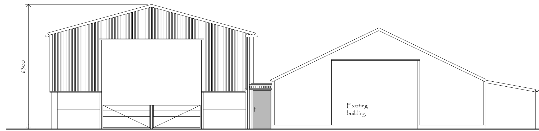
Front [south]
