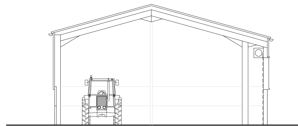
Section B-B
