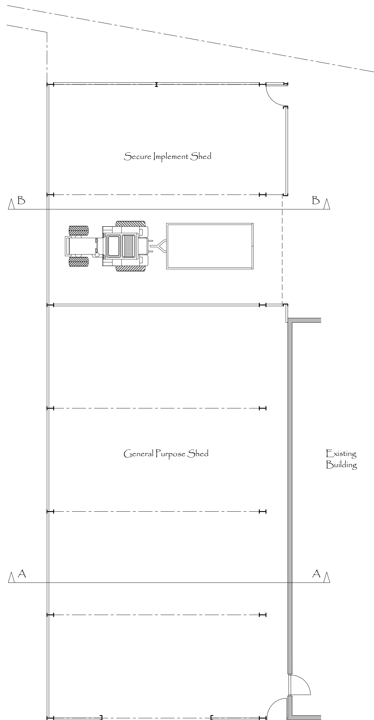
Plan
