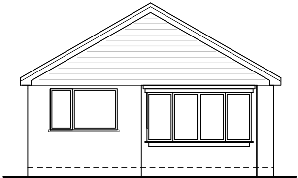
front (southeast) elevation
