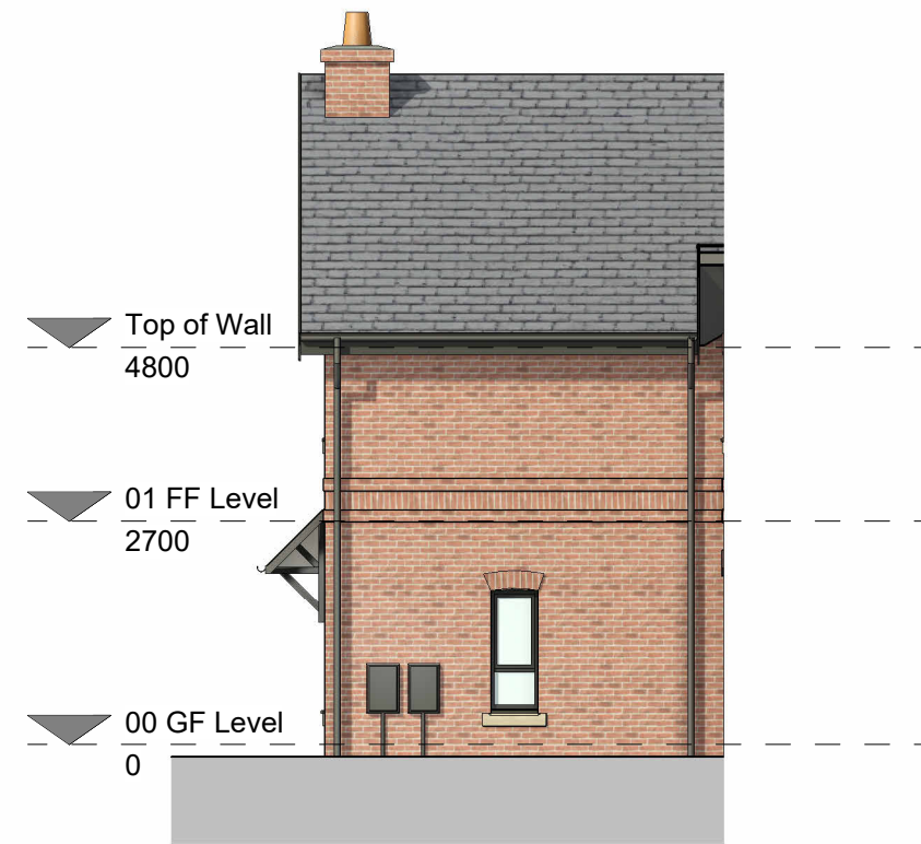
Interior West Elevation 1 : 100
