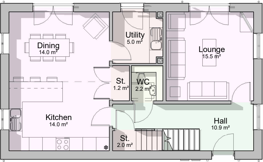
Ground Floor 1 : 100
